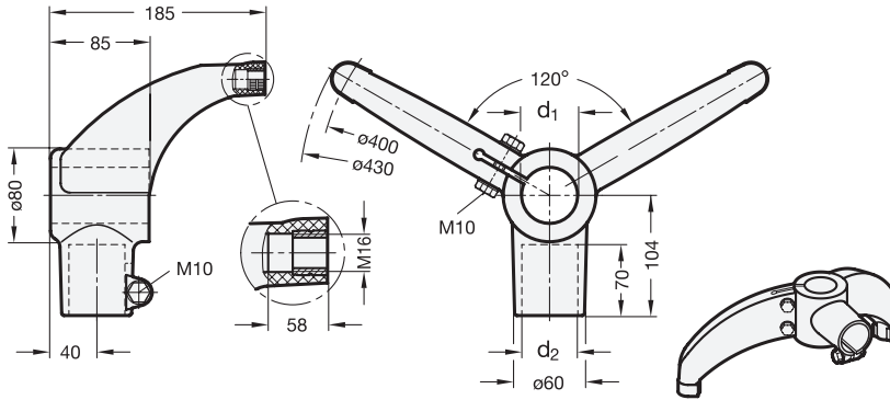
ELESA Original design BAG2-120
