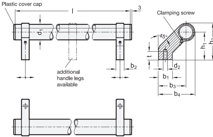
3 Type A Mounting from the back (threaded blind bore)
