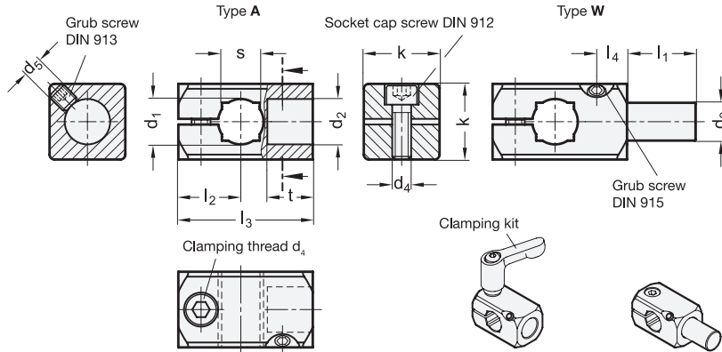
Type A with bore W with bolt
