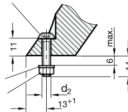
Socket button head screw
