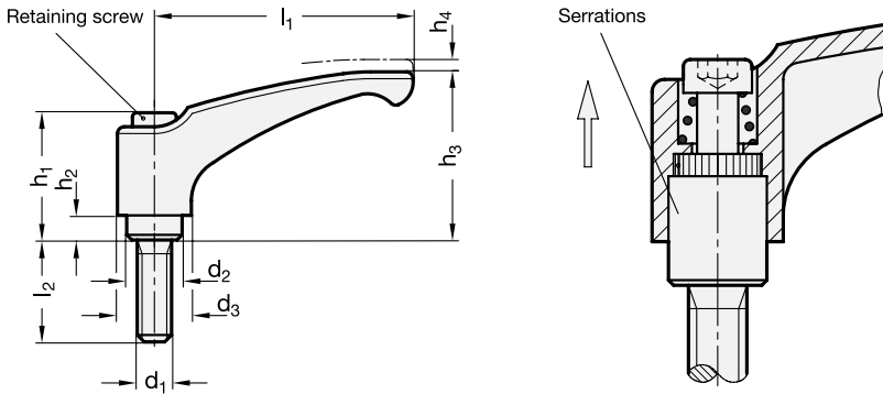
ELESA Original design ERM.SST-p
